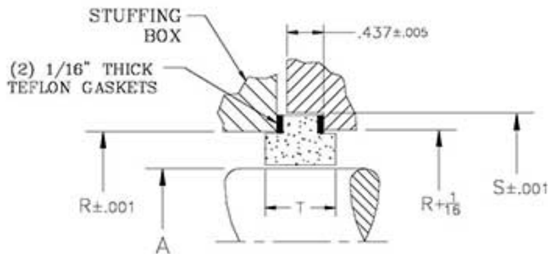
FLEX-A-SEAL STYLE 02
